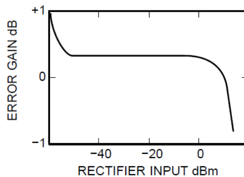
Figure 10. Rectifier Accuracy
