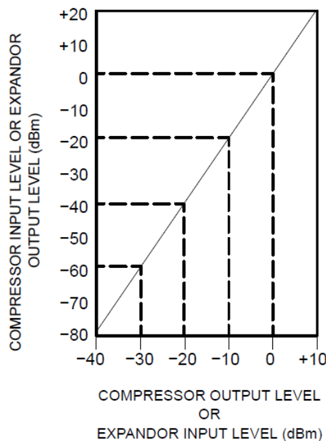
Figure 2. Basic Input-Output Transfer Curve
