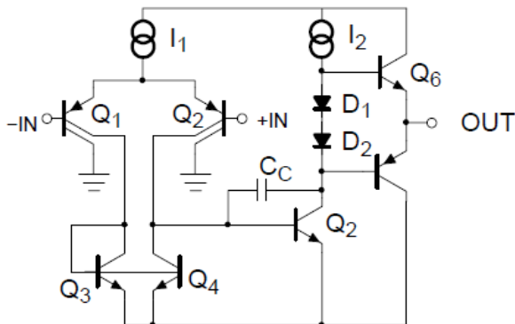
Figure 17. Operational Amplifier
