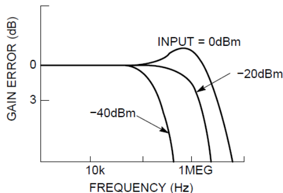
Figure 11. Rectifier Frequency Response vs. Input Level
