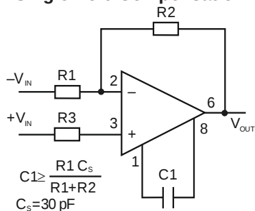
Single Pole Compensation
