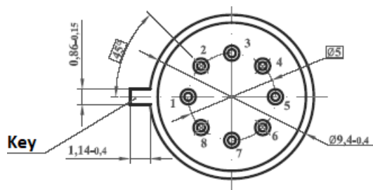
AS301AH Bottom view
