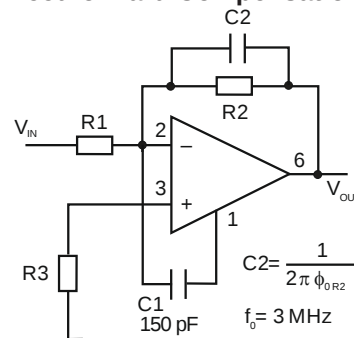
Feedforward Compensation
