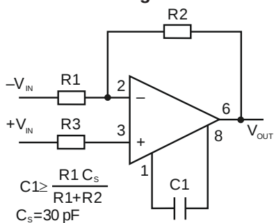
Balancing Circuit
