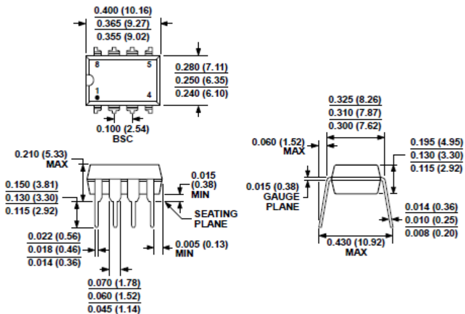
Figure 16. 8-Lead Plastic Dual In-Line Package (PDIP)
