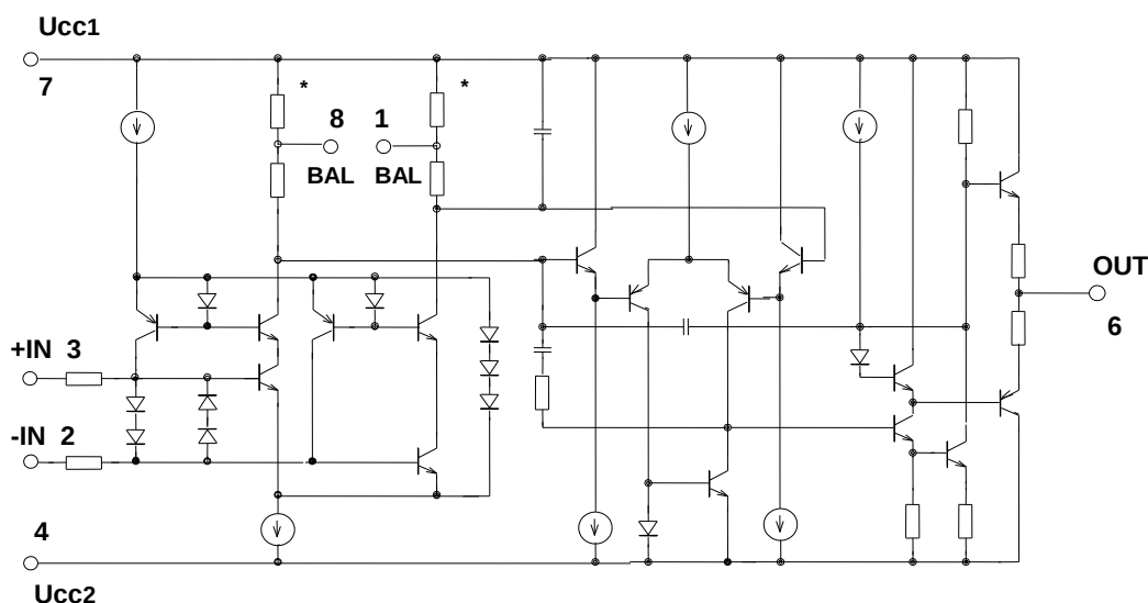
Figure 15. Simplified Schematic
