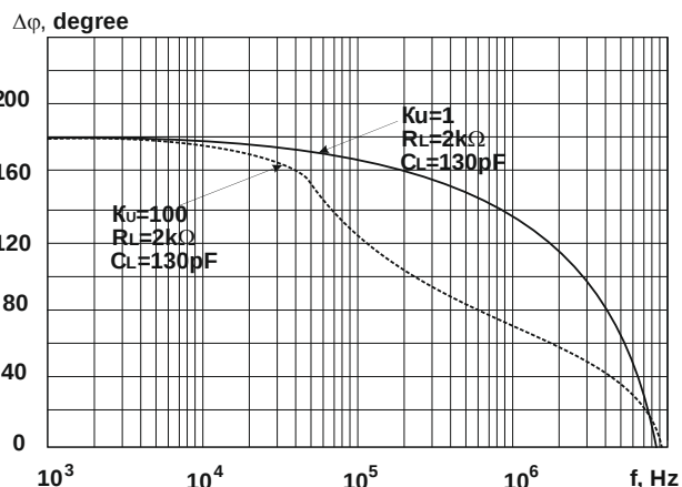
Fig. 6 Phase-frequency response for various feedback gain
