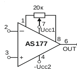
Fig. 12 Balancing scheme
