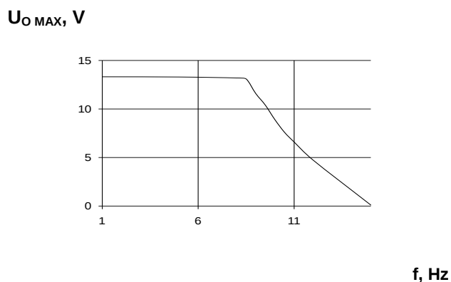
Fig. 8 The dependence of the maximum output voltage on the frequency
