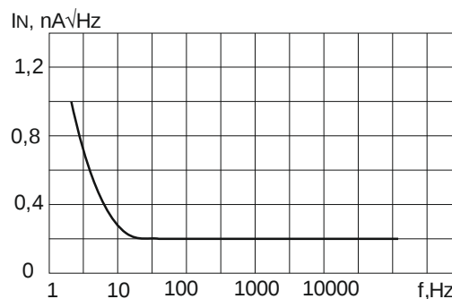
Fig. 10 The dependence of the spectral density of the noise current on the frequency
