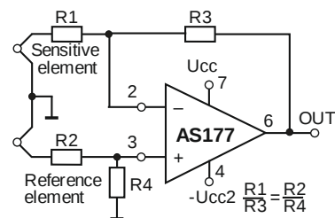
Fig. 14 Highly stable thermocouple amplifier
