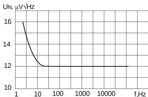
Fig. 9 Frequency dependence of the spectral density of noise voltage
